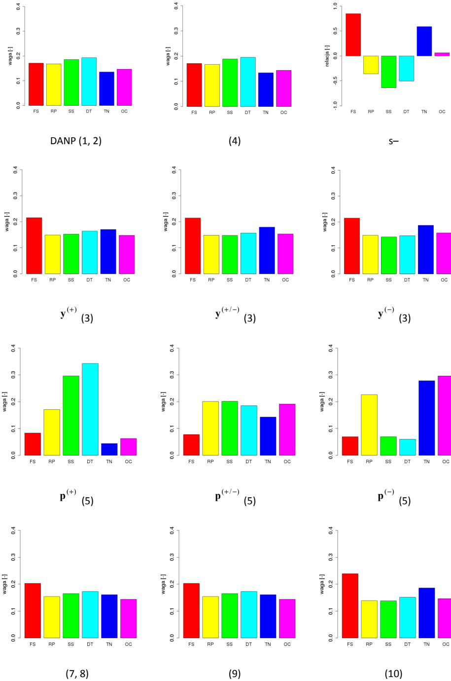
Fig. 3 Comparison of the results of the various techniques of weighting and ranking of factors
